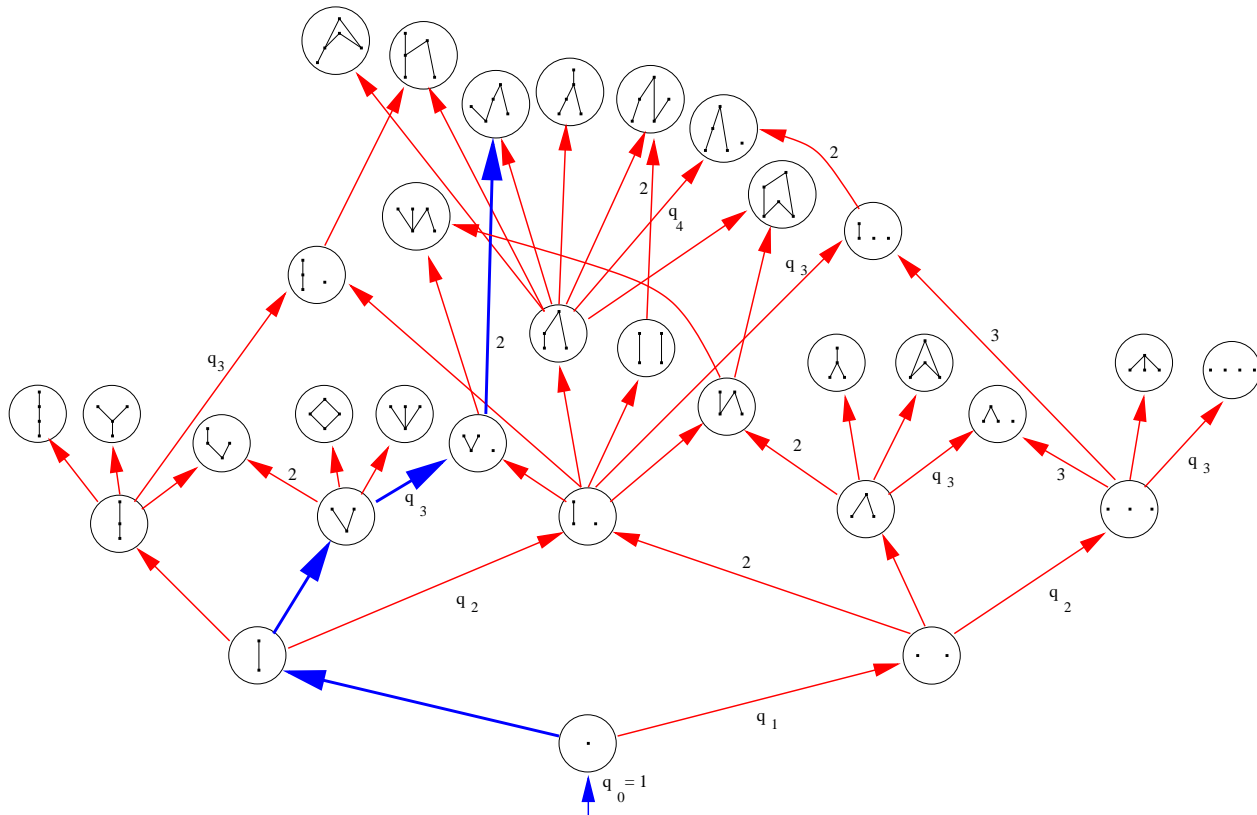
Figure 1: The poset of finite causets
